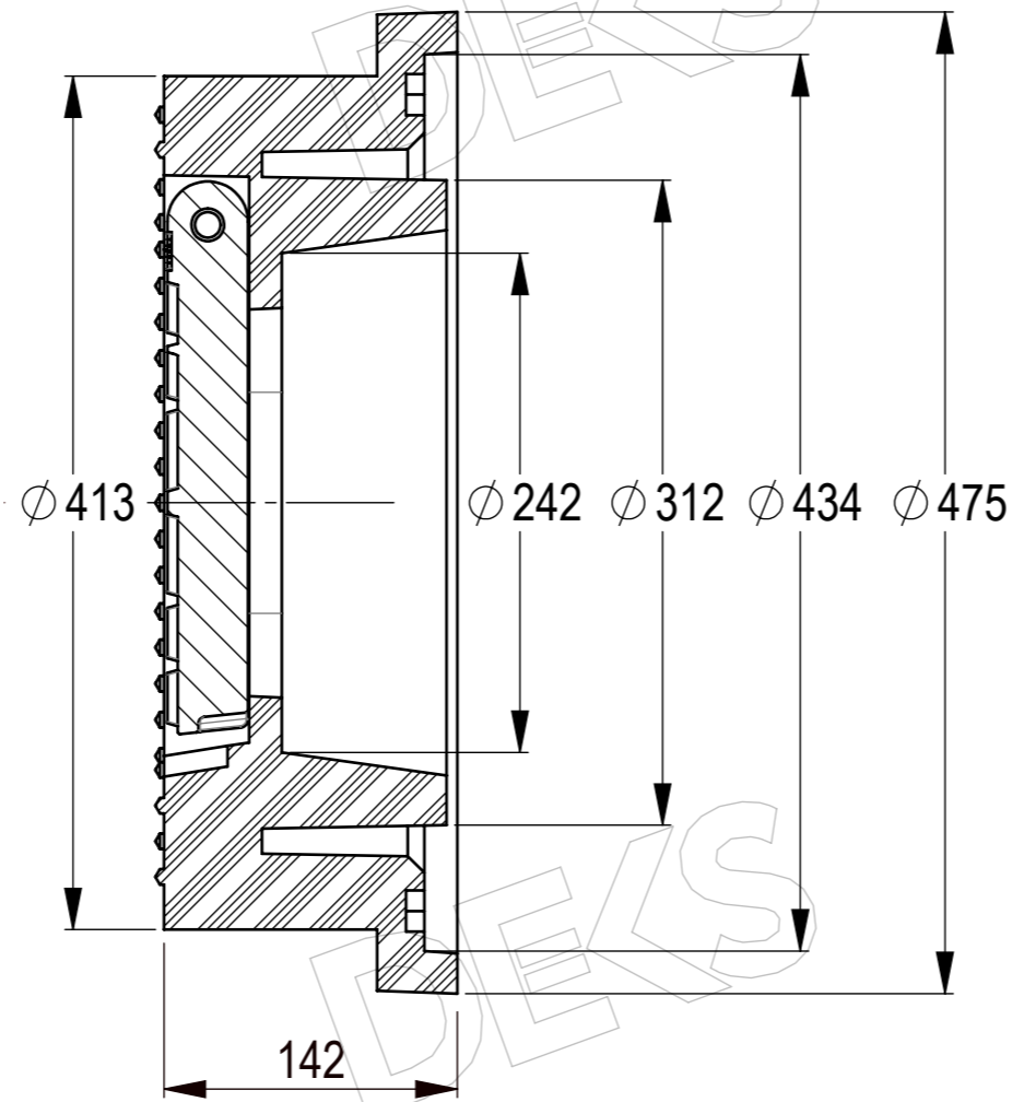
SECTION 'A'-'A'
